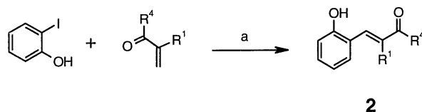
Scheme 3. (a) \text{Pd}(\text{OAc})_2 , \text{NaHCO}_3 , (n\text{-Bu})_4\text{NI} , DMF, 60^\circ\text{C} (11–45% yields).
