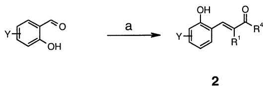
Scheme 2. (a) \text{R}^1\text{CH}_2\text{C}(\text{O})\text{R}^4 , NaOH, \text{H}_2\text{O} , rt (15–97% yields).
