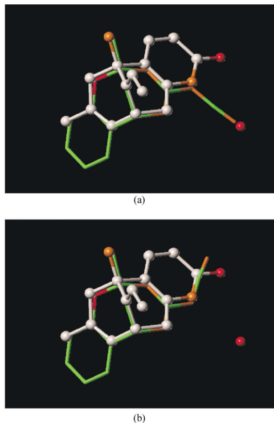
Figure 7. (a) Overlap of Compound 1a (green) and Huperzine A (silver) with Z-configuration assumed for double bond. (b) Overlap of Compound 1a (green) and Huperzine A (silver) with E-configuration assumed for double bond.
