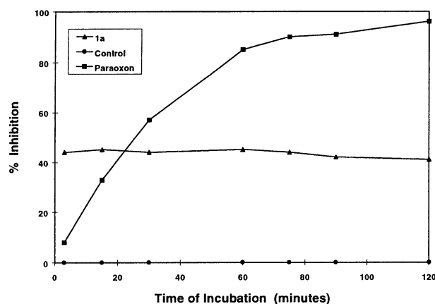
Figure 4. Time-course of inhibition of AChE from Southern corn rootworm ( Diabrotica undecimpunctata ) by 1a or paraoxon. AChE from Southern corn rootworm was incubated for up to 120 min with 2 \mu\text{M} 1a or 300 nM paraoxon. The concentrations chosen were approximately equal to the I_{50} measured for each compound in dose-response experiments. The control AChE preparation was incubated similarly, except for the lack of exposure to either compound. Each data point represents the mean of triplicate determinations. The SEM was typically less than 5%.
