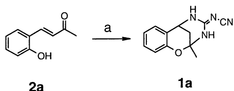
Scheme 1. (a) \text{H}_2\text{NCN} (2 equiv), piperidine (cat), DME, reflux ( 1a , 46%).
