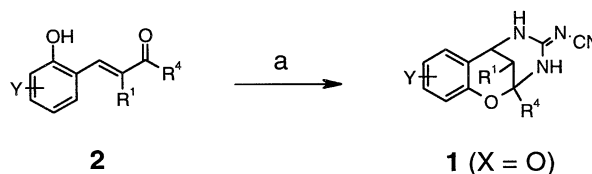
Scheme 4. (a) \text{H}_2\text{NCN} (2 equiv), piperidine (cat), DME, reflux (3–85% yields).
