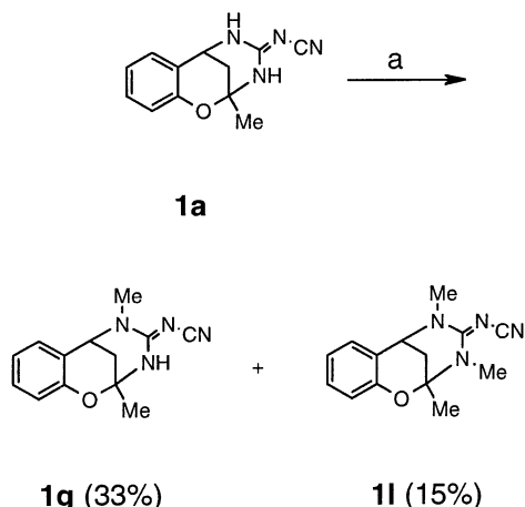
Scheme 6. (a) NaH (2.2 equiv), MeI, (4 equiv), DMF, rt.
