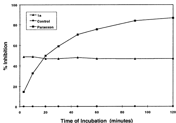
Figure 5. Time-course inhibition of AChE from Green leafhopper ( Nephotettix cincticeps ) by 1a and paraoxon. AChE from Green leafhopper was incubated for up to 120 min with 3 \mu M 1a or 1 \mu M paraoxon. The concentrations chosen were approximately equal to the I_{50} measured for each compound in dose-response experiments. The control AChE preparation was incubated similarly, except for the lack of exposure to either compound. Each data point represents the mean of triplicate determinations. The SEM was typically less than 5%.
