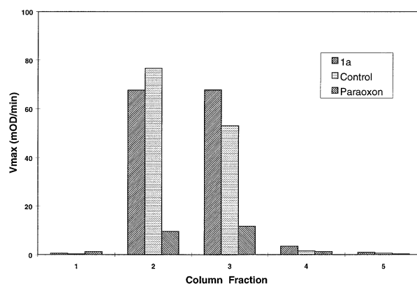
Figure 6. Molecular size-exclusion chromatography of AChE from Southern corn rootworm ( Diabrotica undecimpunctata ) treated with 1a or paraoxon. Identical Sephadex G-25-300 columns were poured with bed volumes of approximately 10 mL. The columns were equilibrated with 0.1 M sodium phosphate, pH 7.4. Next, a 3 mL aliquot of AChE was mixed with 1a (10 \mu M final concentration), paraoxon (1 \mu M final concentration) or dimethyl sulfoxide (solvent control). The enzyme-inhibitor mixture was incubated for 30 min at 23 °C. Following incubation, 2 mL of each mixture was loaded onto separate columns and eluted with sodium phosphate buffer. Five 2 mL fractions were collected with 20 \mu L aliquots taken from each fraction and assayed in the standard AChE assay. AChE assay conditions were identical to that in Methods except: no additional solvent or compound was added to the well, 190 \mu L of buffer was used, the microplate was not incubated prior to ATC/DTNB addition.
