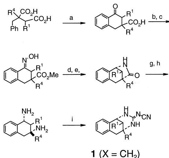
Scheme 7. (a) H_2SO_4 ; (b) MeOH, HCl, reflux; (c) NH_2OH ; (d) H_2 (50 psi), PtO_2 , MeOH; (e) 120^\circ C , 4 h; (f) separate diastereomers (when R^1 , R^3 other than H); (g) HCl, reflux; (h) HN_3 ; (i) (PhO)_2C=NCN , i -PrOH, reflux.
