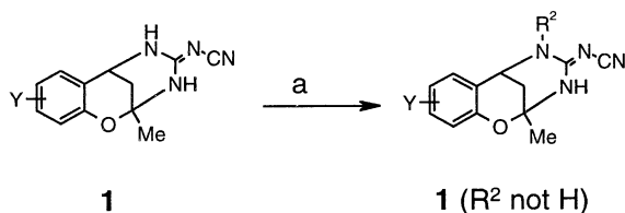
Scheme 5. (a) NaH (1.1 equiv), R^2 -X, (1.1 equiv), DMF, rt.
