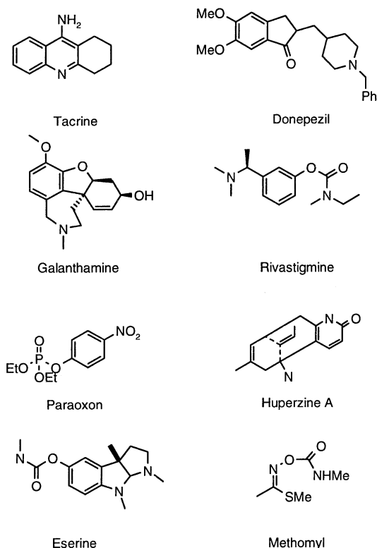
Figure 1. Acetylcholinesterase (AChE) inhibitors.
